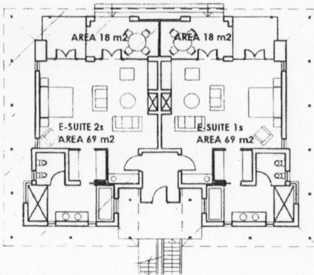
UNIT E: Ground Floor Plan
